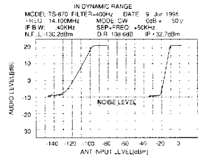
Figure 22: Dynamic range
