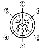
Rear Panel view on TS-450S/690S/850S/950SDX
